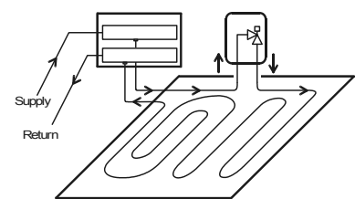
Fig. 6. Room Control-Set (supply)
