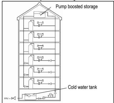
Diagram 6 Multi-storey pump-boostered with high and low storage
