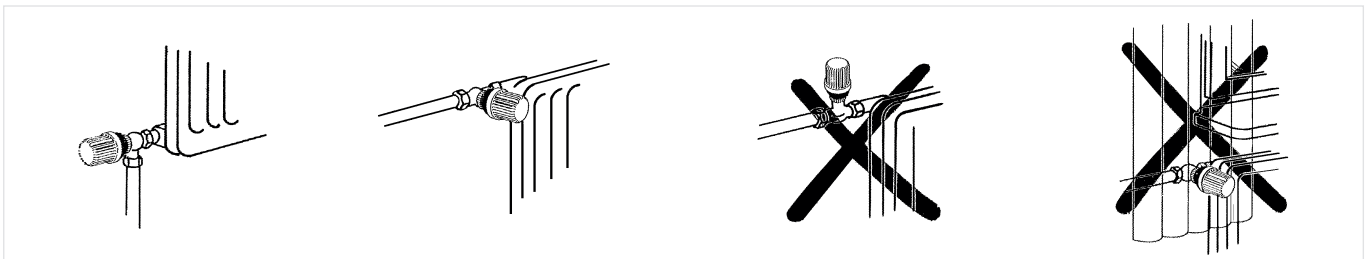
Fig. 2 Correct and false installation positions for radiator thermostats with internal sensor
