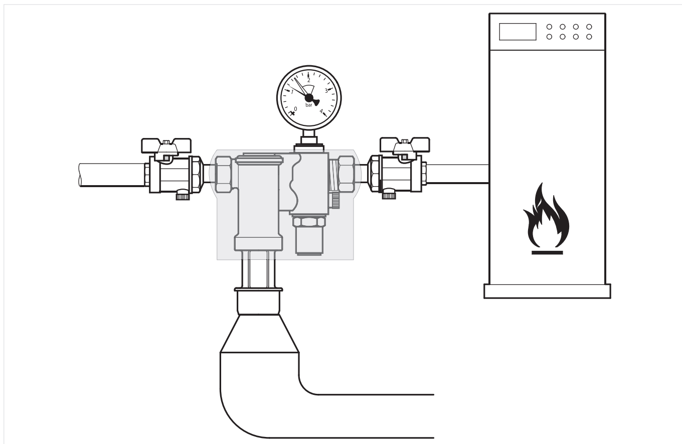
Fig. 1 Standard installation example for the refilling combination
