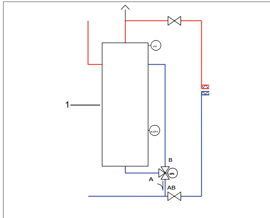
1 Buffer tank
